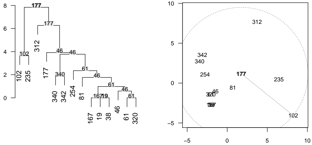
Figure 3: View of a subtree (left) from Fig. 2a with the branch's prototype in bold and prototypes associated with each leaf (labels are row indices of data points in the original data set) and representation of dissimilarities (right) via multidimensional scaling (minimax linkage is the radius drawn on the plot)
