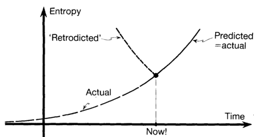
Figura 1: The initial statistical explanation by Boltzmann was insufficient, due to the reversibility problem, since the explanation also predicts an entropy increase towards the past.
