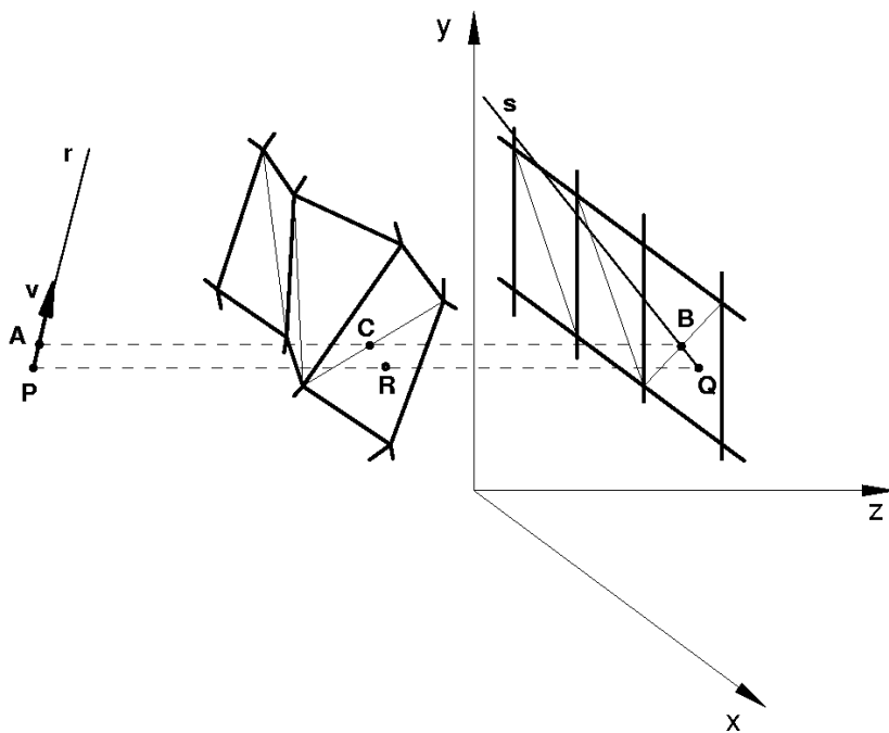
Figure 3: Trajectory, surface, and their projections.
