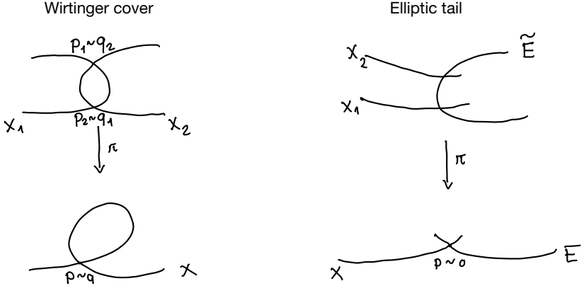
Figure 2: Stable covers
