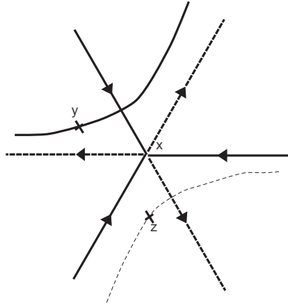
Figure 2: At the singular point x the stable manifold through y does not intersect the unstable one through z .
