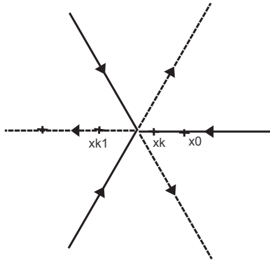
Figure 3: The pseudo orbit consisting of the f past of x_k and the f -future of x_{k+1} ( x_{k+1} very close to x_k ) is not shadowed by an f -orbit (see fig. 1)
