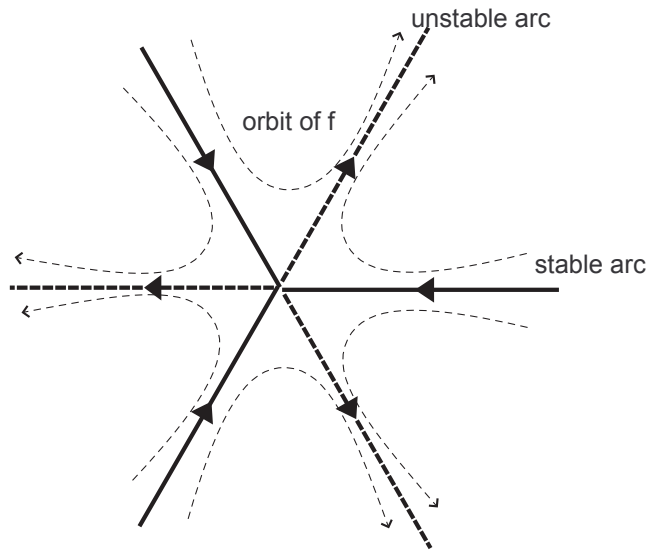
Figure 1: A singular point x of a pseudo-Anosov map f and nearby orbits.
