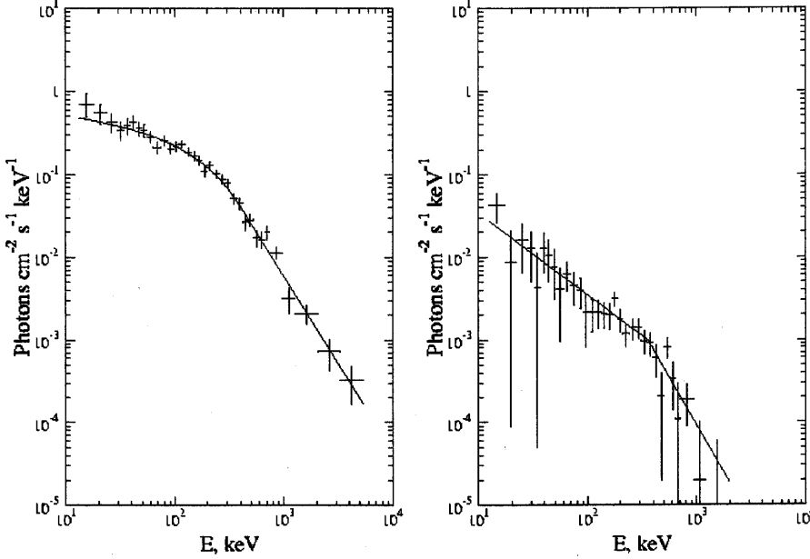
Figure 1.4: Two typical GRBs energy spectra.
