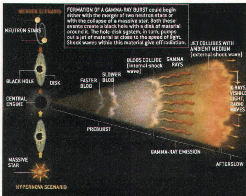
Figure 1.5: Schematic representation of the mechanisms producing a long GRB and its afterglow in the framework of the fireball model. The left part of the Figure and the inset refer to two possible progenitors of the fireball that are discussed in Par. 1.2.3.
