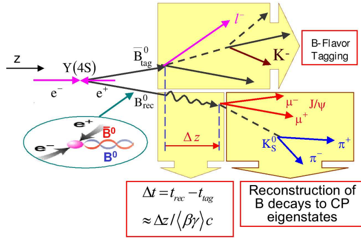
Figure 4.2: An illustration of the B^0\bar{B}^0 decays used to extract time-dependent CP asymmetries. B_{rec} is fully reconstructed and the remaining particles are used to infer the flavor of B_{tag} . The time-difference between the two B decays is determined from the separation of the decay vertices.
