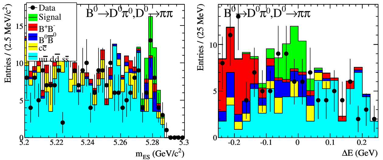
Figure 3.9: m_{ES} and \Delta E distributions for the data (points) and generic MC (histograms) for \bar{B}^0 \rightarrow D^0 \pi^0 where D^0 \rightarrow \pi^+ \pi^- . High background contamination can be seen in the signal region. For this reason this mode was excluded from the time-dependent final fit.
