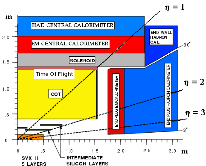
Figure 3.5: One quadrant of the CDF detector tracking layout.
