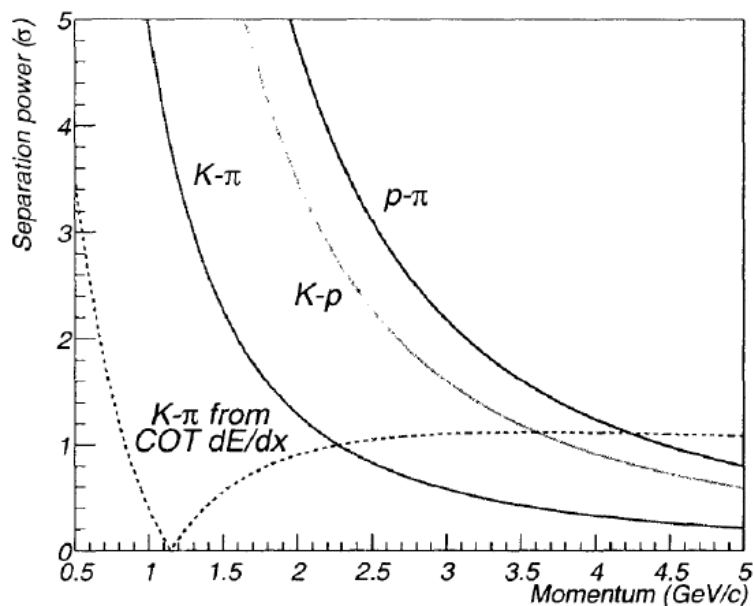
Figure 3.10: Separation power of TOF for different particles at CDF, with dE/dx separation power for kaon and pion from COT superimposed.
