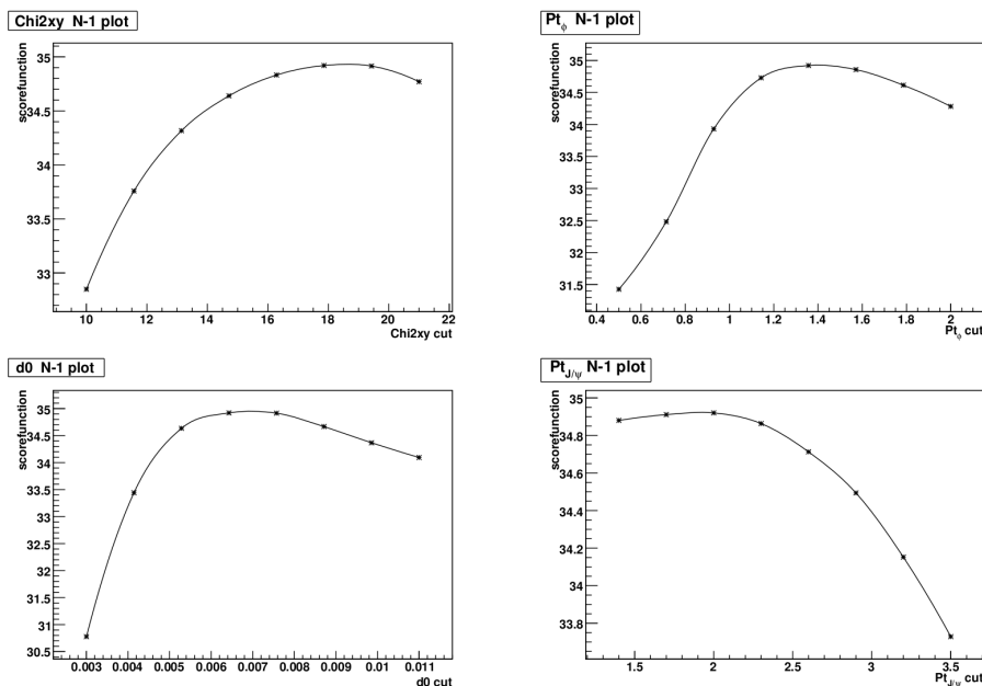
Figure 6.6: N - 1 plots of the score-functions as a function of the variable cuts for the B_s \rightarrow J/\psi\phi decay. From top to bottom, left to right the variables are: the B_s meson \chi_{xy}^2 , the \phi the transverse momentum, the B_s meson impact parameter, the J/\psi transverse momentum.
