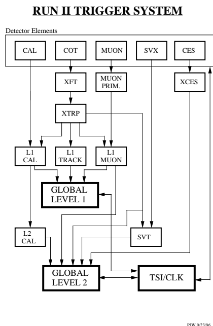
Figure 3.14: CDFII Trigger structure.
