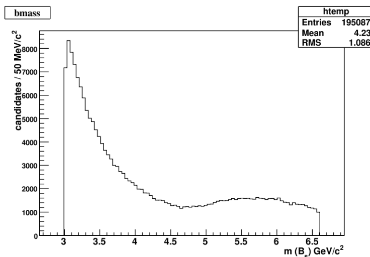
Figure 6.2: B_s invariant mass distribution after the preselection.
