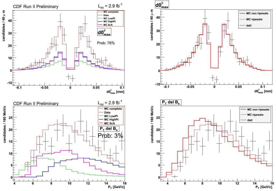
Figure 5.2: Data-Monte Carlo comparison similar to that of Figure 5.1, for the distributions of the impact parameter of \phi with higher energy and of the p_T of B .
