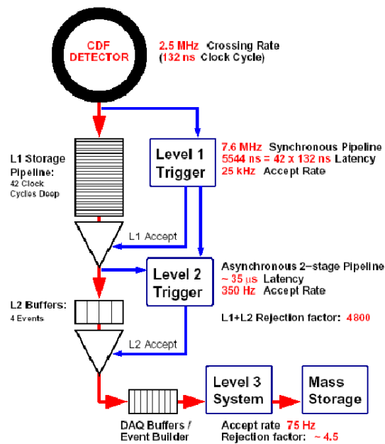
Figure 3.13: CDF Trigger decisions tree flow.
