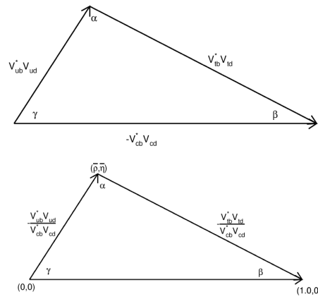
Figure 2.3: Illustration of db unitarity triangle (top), and rescaled db unitarity triangle (bottom) with \tilde{\rho}\tilde{\eta} defined
